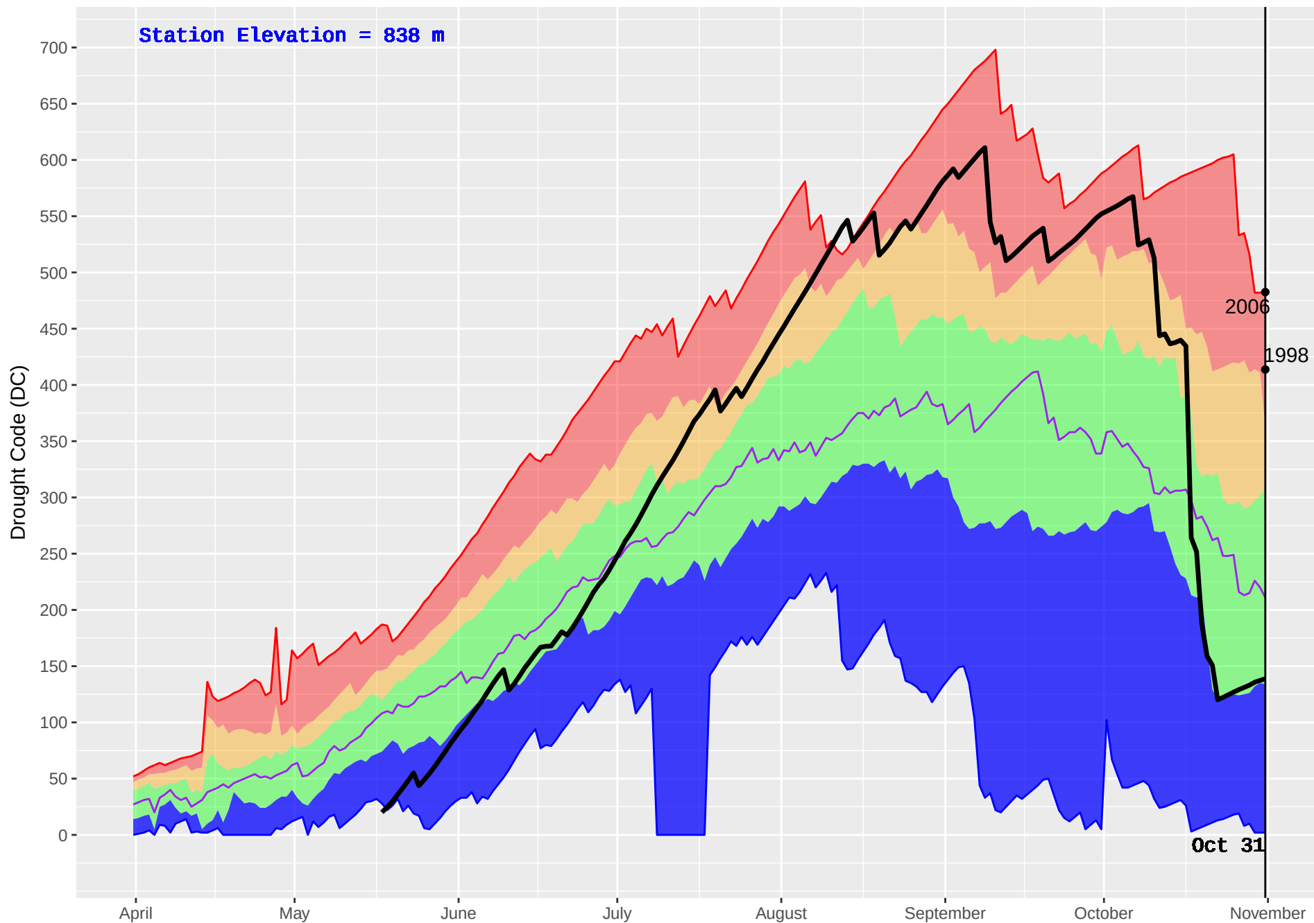
HOWARD (343) : Historical (1970–2016) and Current (2017) Noon Drought Code (DC)
